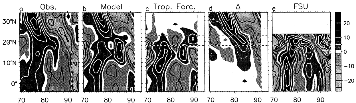
part of Figure 1. (b) Same as (a) but from results of an oceanic circulation model (Venzke 1999) forced with observed anomalies of surface wind stress (Da Silva et al. 1994), heat flux (Da Silva et al. 1994) and surface temperature (Parker et al. 1995). (c) Results from an experiment in which the anomalous atmospheric forcing was restricted to the area equatorward of 18^{\circ} latitude. To avoid artificially generated curl of the wind stress a linear transition to zero anomalous forcing extended from 18^{\circ} to 23^{\circ} latitude (indicated by dashed lines). (d) Difference of 25.5 \text{ kg m}^{-3} \sigma_{\theta} isopycnal depth anomalies of simulations with full forcing (b) and tropical forcing (c). The additional dotted contours mark differences with magnitudes of 3 m. (e) Depth anomalies obtained by forcing the ocean general circulation model with wind stress anomalies assembled by the Florida State University (Stricherz et al. 1992, 1997). Anomalous wind stress was estimated from the pseudo-stress by a constant drag coefficient of 10^{-3} . As in (c) wind-stress anomalies were applied within 18^{\circ} latitude of the equator, and ramped to zero at 23^{\circ} latitude. In all plots the contour interval is 5 m, light shading denotes negative depth anomalies, corresponding to a shallowing of the isopycnal, and dark shading represents positive depth anomalies (see the gray-scale on the right). The vertical dotted lines in (a) to (d) mark the end of the model experiment. All results have been smoothed using a low-pass filter with a half power at 6.7 years.
